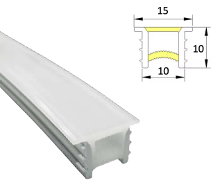
Silicone Cover SY1010
