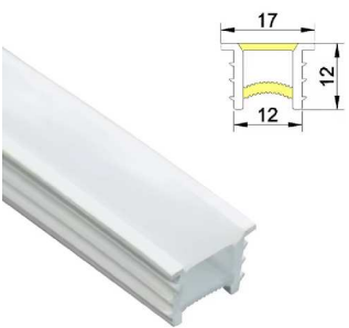
Silicone Cover SLY1212
